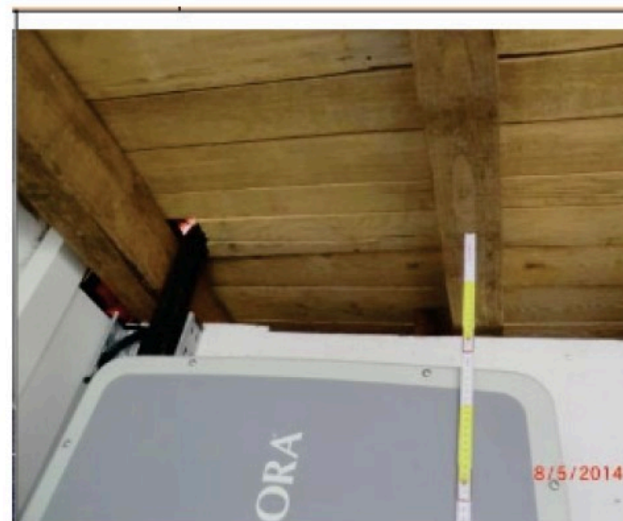
Distance to bottom, top or to the sides too low [By courtesy of TUV Rheinland].
