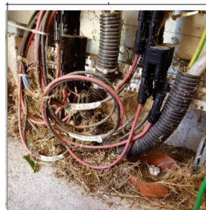
Presence of inflammable mate- rial [By courtesy of SUPSI PVLab].
