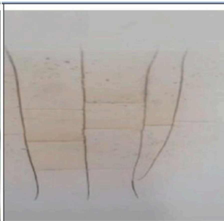
Cracked backsheet in combination with yellowing under a hot cell [Eder19].
