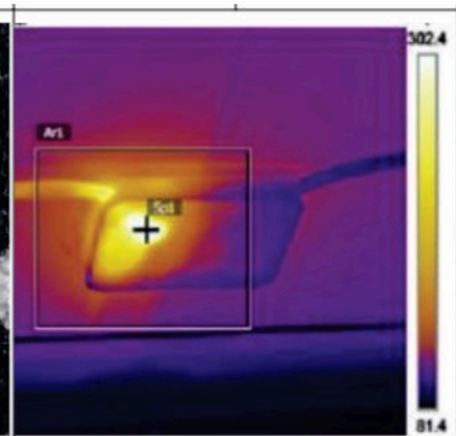
IR imaging of a hotspot Jbox due to loose electric connection inside [Yang19].
