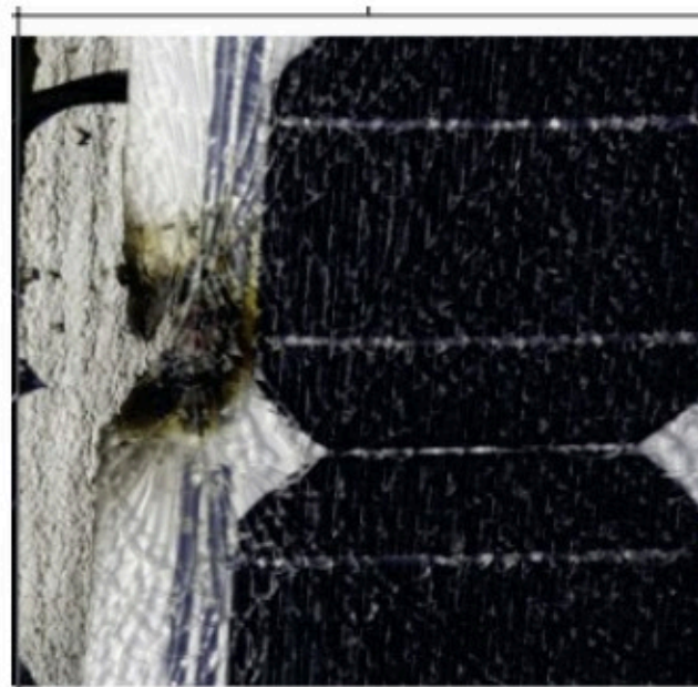
Overheating due to the poor Jbox interconnect leading to burn mark and glass breakage [Yang19].
