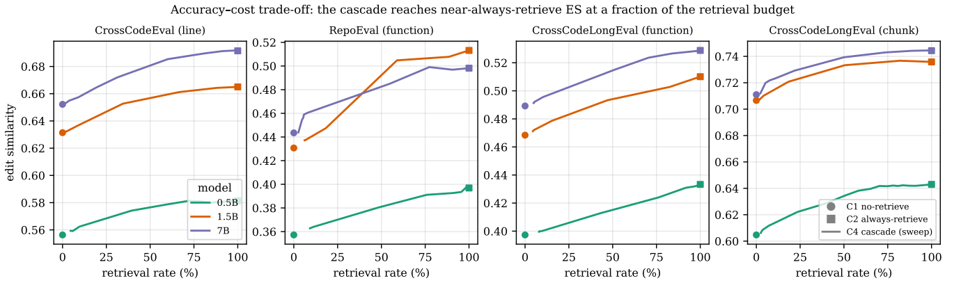
Fig. 3. Accuracy-cost trade-off (RQ2). Edit similarity vs. retrieval rate as T_{\text{RAG}} is swept (C4 cascade); \bullet = \text{C1} , \blacksquare = \text{C2} . The \text{C1} \rightarrow \text{C2} gain is modest in our setup, and the selective frontier captures it well below a 100% retrieval budget, for all three models and all four surfaces.
