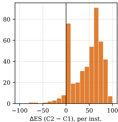
RepoEval (function) helps 86% · hurts 4% · ~same 10%
