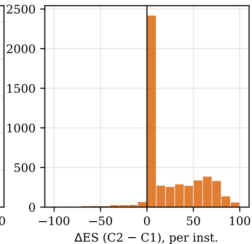
CrossCodeLongEval (chunk) helps 53% · hurts 4% · ~same 42%
