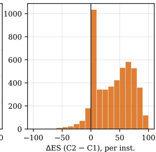
CrossCodeLongEval (function) helps 80% · hurts 7% · ~same 13%
