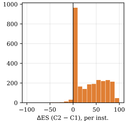
CrossCodeEval (line) helps 66% · hurts 2% · ~same 32%
