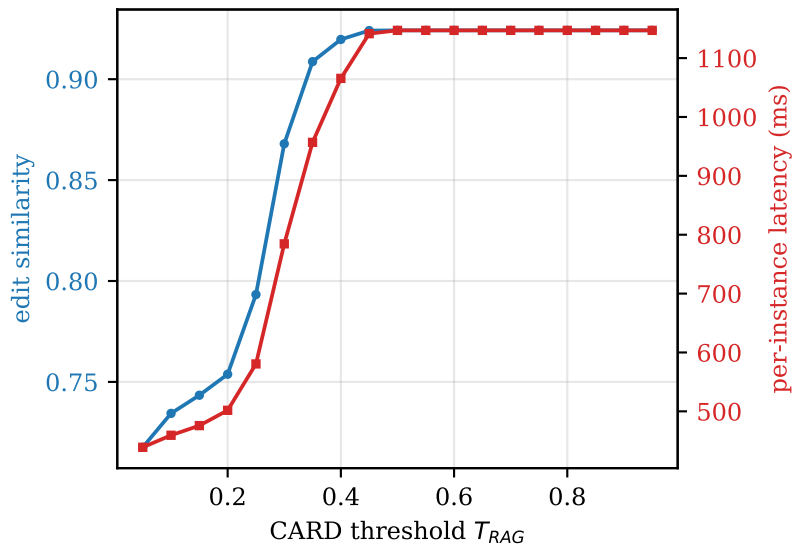
CrossCodeLongEval (chunk) \cdot 7B
