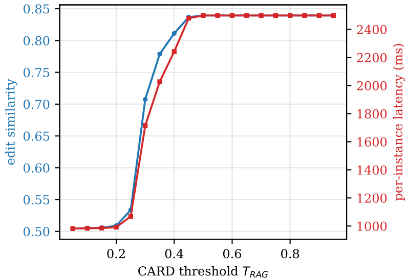
CrossCodeLongEval (function) \cdot 7B
