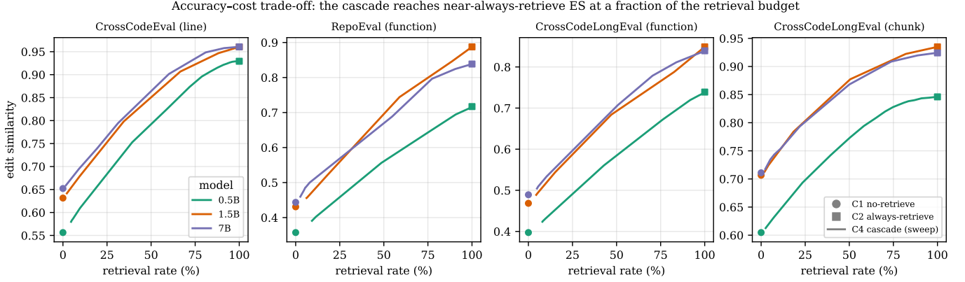
Fig. 3. Accuracy-cost trade-off (RQ2). Edit similarity vs. retrieval rate as T_{\text{RAG}} is swept (C4 cascade); \bullet = C1, \blacksquare = C2. The selective frontier reaches near-C2 accuracy well below a 100% retrieval budget, for all three models and all four surfaces.
