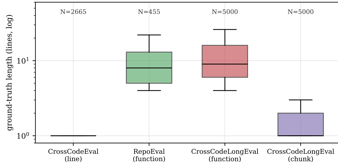
Completion-target length by benchmark (whiskers: 5-95th pct)
