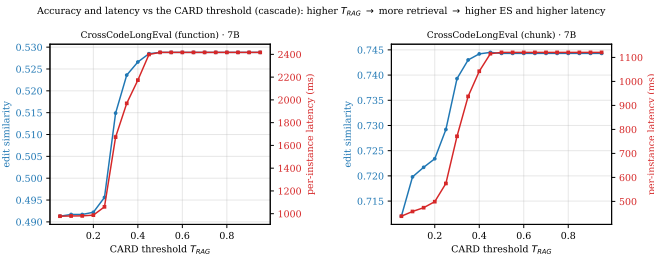
Fig. 4. Accuracy and latency vs. the CARD threshold (7B cascade): both rise with T_{\text{RAG}} and plateau, so the threshold is a single knob trading per-instance latency for accuracy (RQ2).
