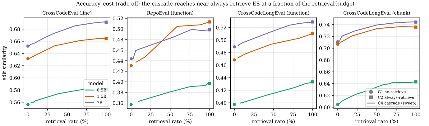
Fig. 3. Accuracy-cost trade-off (RQ2). Edit similarity vs. retrieval rate as T_{\text{RAG}} is swept (C4 cascade); ● = C1, ■ = C2. The selective frontier captures the C1→C2 gain well below a 100% retrieval budget, for all three models and all four surfaces.
