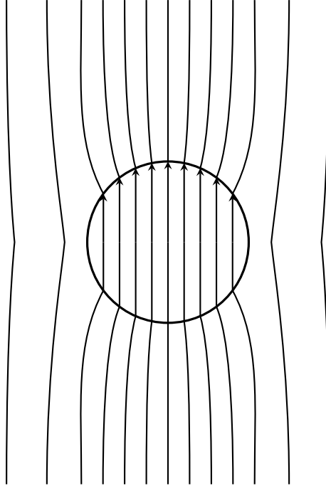
Figure 1. Electric field lines for a dielectric sphere ( \varepsilon_r = 3 , a = 1 ) in a uniform applied field \mathbf{E}_0 . Inside the field is uniform and weaker, \mathbf{E}_{\text{int}} = \frac{3}{5} \mathbf{E}_0 ; outside it is the superposition of \mathbf{E}_0 and an electric dipole. Lines refract at the boundary satisfying continuity of E_{\parallel} and D_{\perp} .
