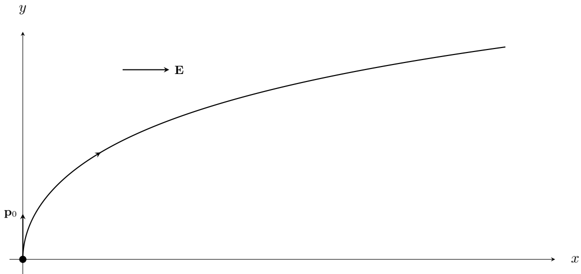
Figure 1. Trajectory of a relativistic charged particle in a uniform electric field \mathbf{E} = (E, 0, 0) , in natural units \mathcal{E}_0/qE = p_0c/qE = 1 . The particle starts at the origin with momentum \mathbf{p}_0 in the y -direction and follows x = (\mathcal{E}_0/qE)(\cosh(qEy/p_0c) - 1) .
