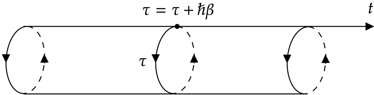
Figure 5. Periodic property of imaginary time, \tau = \tau + \hbar\beta , illustrating the Euclidean time circle that arises in systems at finite temperature.
