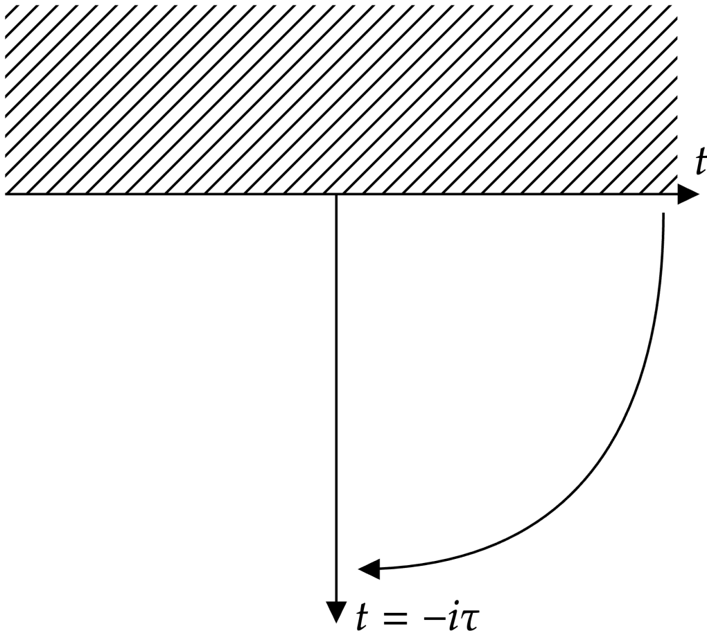
Figure 4. Wick rotation of real time into imaginary (Euclidean) time. The shaded region indicates the domain where evolution is not defined, and the contour is rotated from real time t to Euclidean time t = -i\tau .
