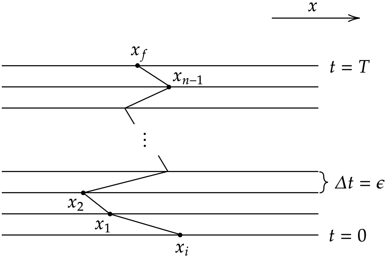
Figure 3. Discretisation of time into n intervals of width \epsilon , with intermediate positions x_1, \dots, x_{n-1} labelling possible segments of a path from the initial point x_i at t = 0 to the final point x_f at t = T .
