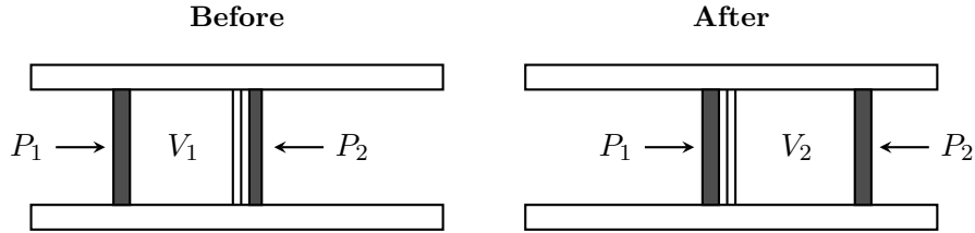
Figure 1. Joule-Thomson process: gas is pushed through a porous barrier from pressure P_1 to P_2 < P_1 .
