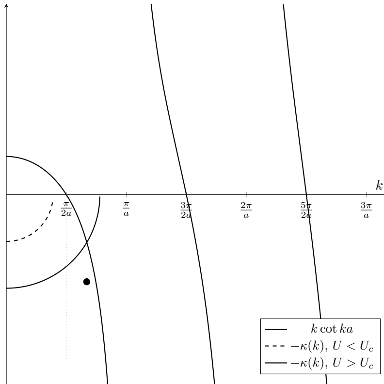
Figure 1. Graphical solution of the odd-parity bound-state equation k \cot ka = -\kappa(k) , where \kappa = \sqrt{2mU/\hbar^2 - k^2} . The dashed semicircle ( U < U_c ) does not intersect k \cot ka — no odd bound state exists. The solid semicircle ( U > U_c ) intersects the first branch (dot) — one odd bound state exists. The critical value is U_c = \pi^2 \hbar^2 / 8ma^2 , at which the circle just reaches k = \pi/2a with \kappa = 0 .
