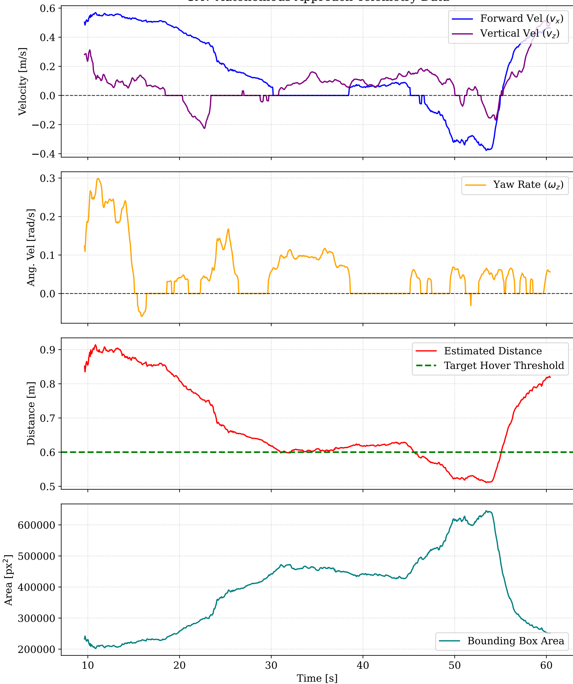
UAV Autonomous Approach Telemetry Data
