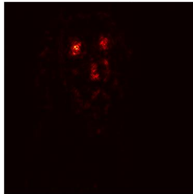
Guided Backprop
