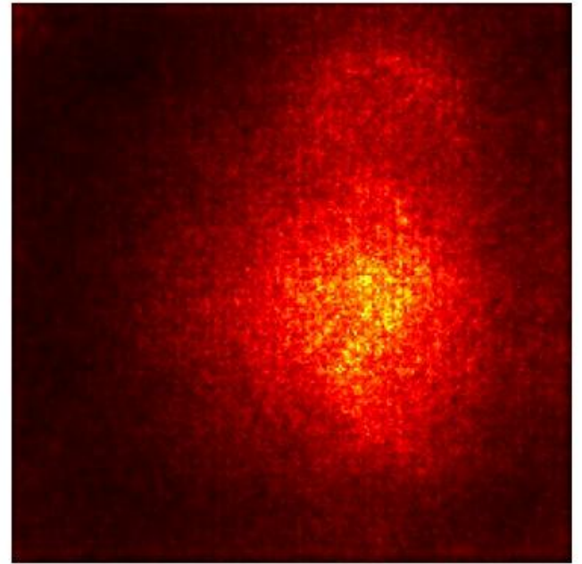
Noise level = 0.5
