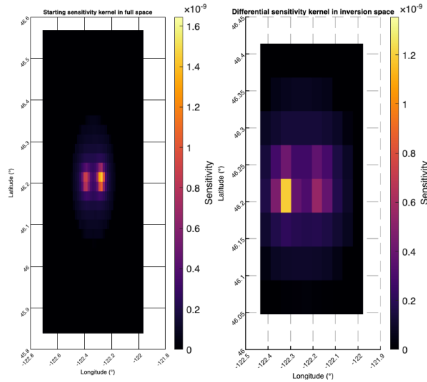
Figure 4.4: (a) Absolute sensitivity kernels measured at the starting time of the coda window t_s = 15 s in the Mount St. Helens case (b) Differential sensitivity kernel between t_e = 25 s and t_s = 15 s.
