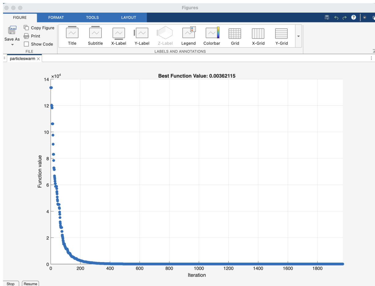
Figure 10.2: Example cost function for the MSH 18 Hz case in the particle swarm inversion.
