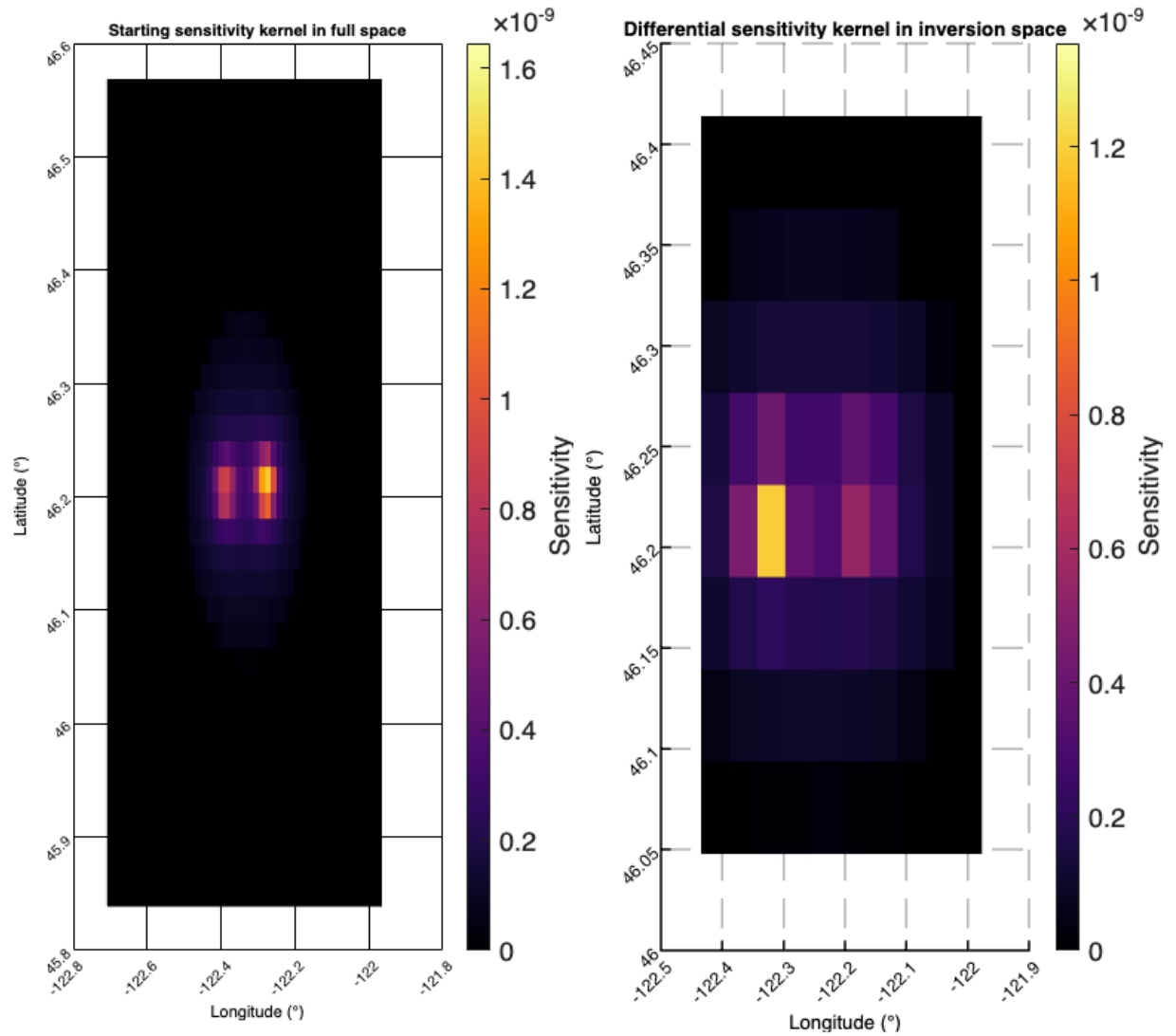
Figure 9.3: Kernels for coda-attenuation imaging at 3 Hz for the MSH dataset. The full kernels are shown as a section in the 3D space (a) and in the grid chosen for the inversion (b). Notice that sensitivity is always highest at the source and receiver. The colour scale is logarithmic. The lapse time is 22.5 s.
