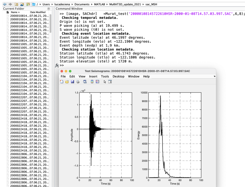
Figure 5.2: Example run of Murat_test . The image is shown while the SACheader is created in the workspace. All the necessary parameters are checked. Notice the missing S-wave picking - the variable storing this parameter may be different from t0 .
