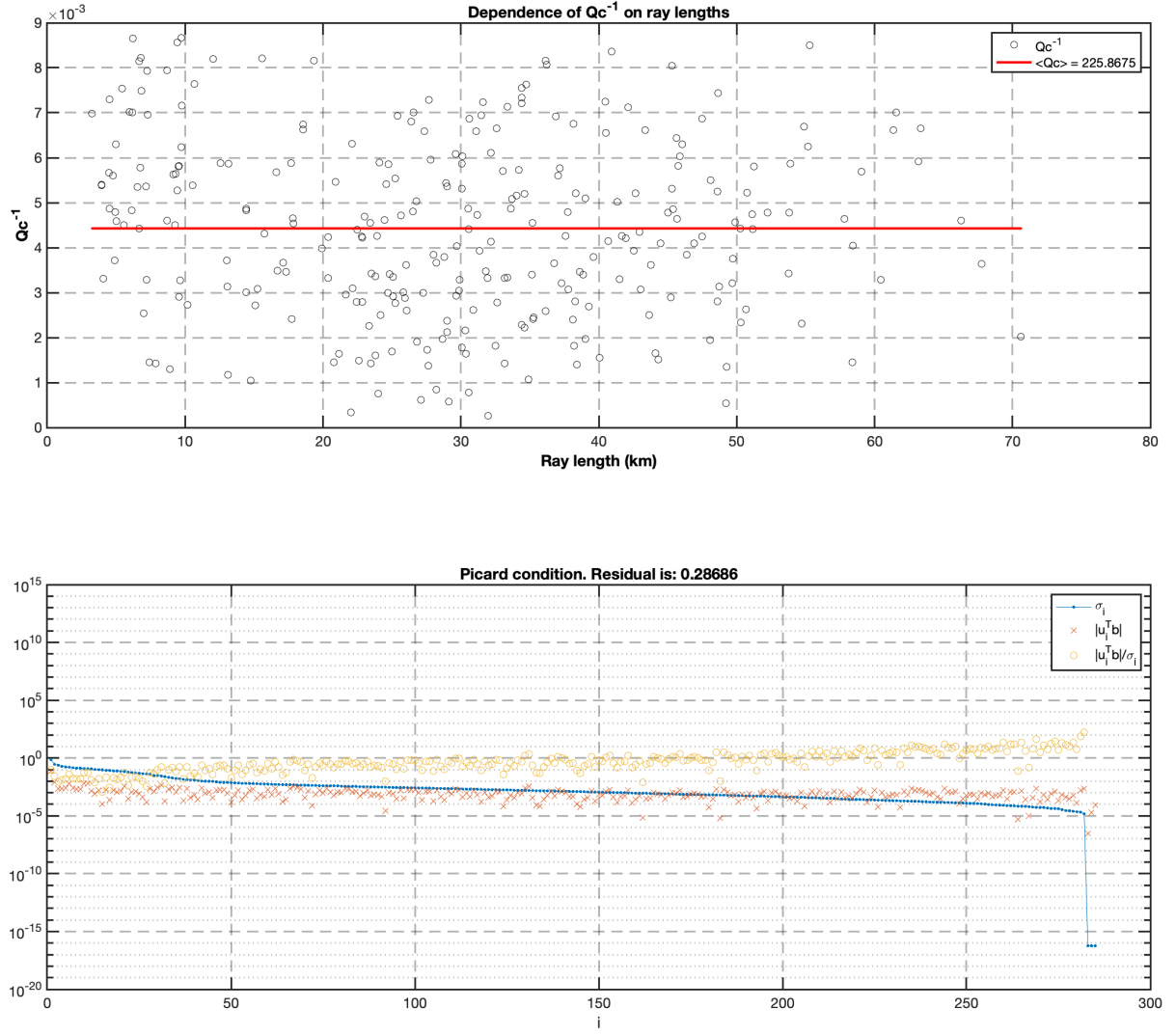
Figure 8.3: Coda analysis plot for the MSH dataset at 6 Hz. The upper panel shows that Q_c is constant with the ray length computed through ray tracing. The lower panel depicts the result of the Picard condition (Aster et al., 2005): only half of the parameter models are solved under the weakest hypothesis (blue and red lines cross around the 150th parameter). Only one-tenth of the parameter models are solved if we also consider the uncertainty of data. \sigma are the singular values.
