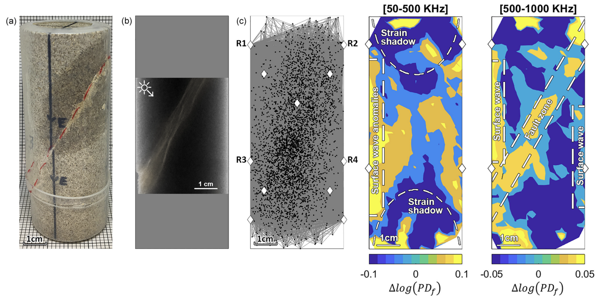
Figure 3.5: Acoustic emission experiment and retrieval of fault zone structure through peak delay imaging, redrawn from King et al. (2022).
