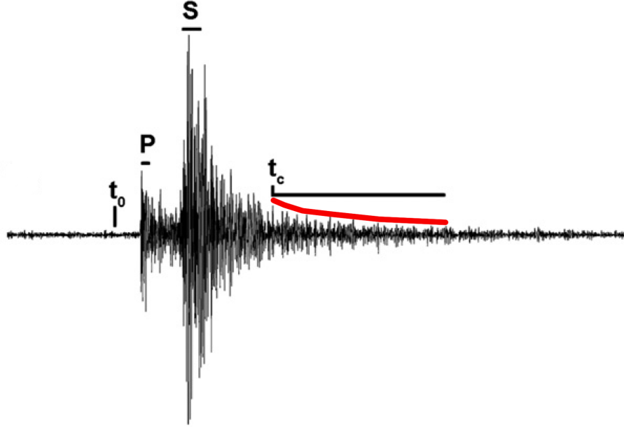
Figure 4.1: The Qc method measures the envelope's decay from a given lapse time from the origin time of the event.
