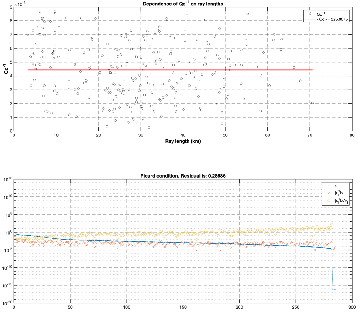
Figure 9.3: Coda analysis plot for the MSH dataset at 6 Hz. The upper panel shows that Q_c is constant with the ray length computed through ray tracing. The lower panel depicts the result of the Picard condition (Aster et al., 2005): only half of the parameter models are solved under the weakest hypothesis (blue and red lines cross around the 150th parameter). Only one-tenth of the parameter models are solved if we also consider the uncertainty of data. \sigma are the singular values.
