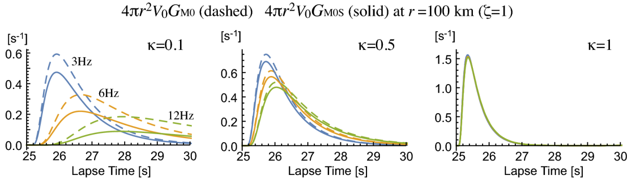
Figure 3.2: Broadening for different \kappa values. For parameters used, see Sato (2016).
