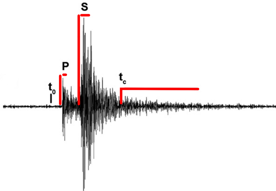
Figure 2.1: The CN method measures the spectral energies of direct and coda waves and inverts for Q . The P and S wave energies, and the normalising coda energies are in red.
