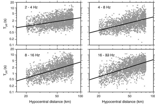
Figure 3.4: Logarithmic plot of peak delay times (in seconds) as a function of the hypocentral distance (in kilometres) for crustal S waves in four frequency bands. Grey dots are the data, and black lines are the regression lines: \log_{10}(T_{pd}) = Ar(f) + Br(f)\log_{10}R . From Calvet et al. (2013).
