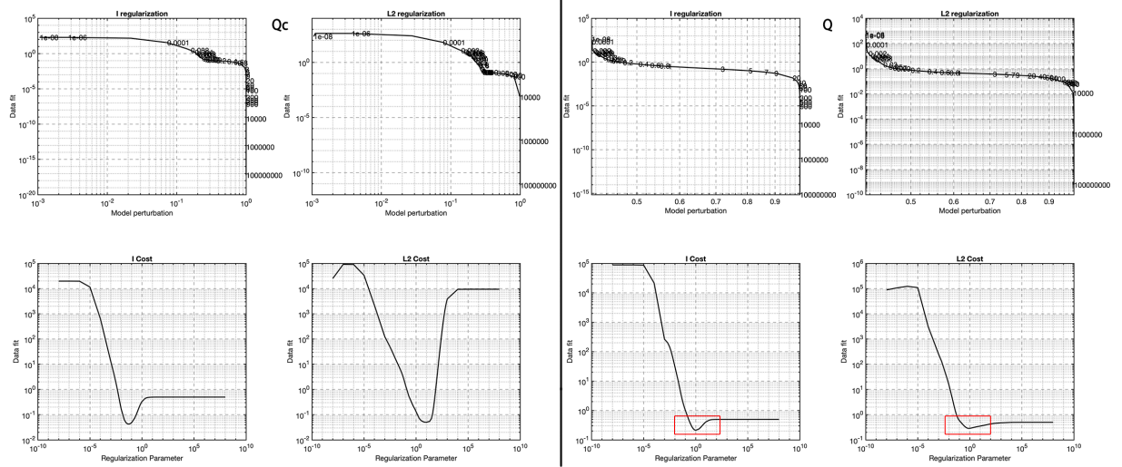
Figure 9.5: Output of the IRTools showing the relation between data fit and either the solution or its smoothness (upper panels, equivalent to the L\_curves ) for the MSH dataset at 6 Hz. The lowermost panels show the corresponding cost function to be minimised. In the case of Q , the cost minimisation parameter (red rectangle) is the same for both conditions.
