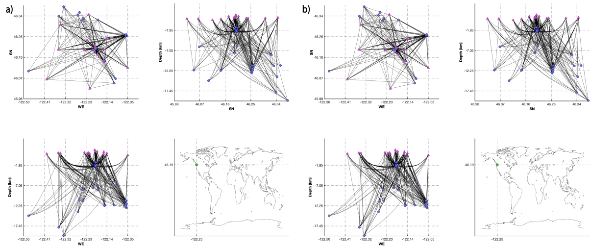
Figure 10.1: Rays of the coda-normalisation (a) and peak delay (b) methods at 3 Hz for the MSH dataset.
