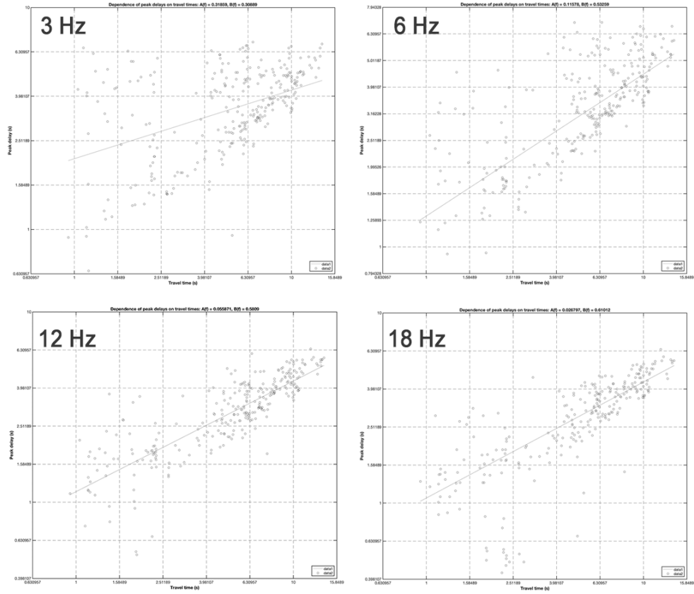
Figure 9.1: Comparison between peak delays for the four frequencies and the Mount St Helens dataset.
