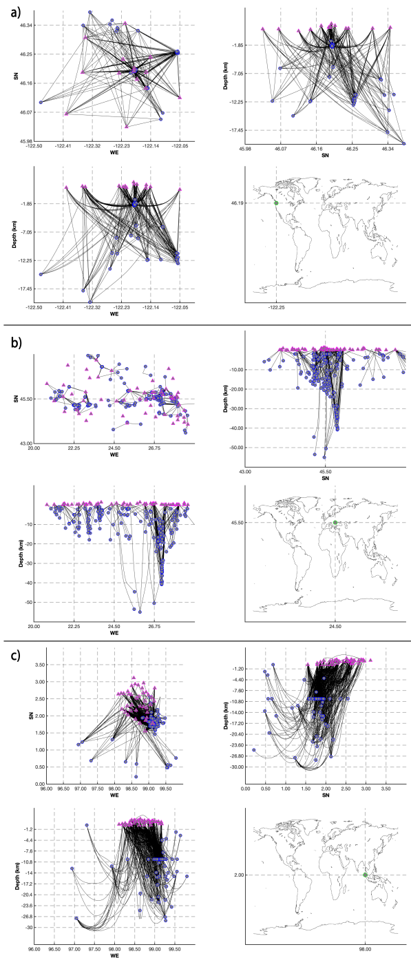
Figure 10.2: Rays of the coda-normalisation method at 3 Hz for the three sample datasets: (a) MSH; (b) Romania; (c) Toba.
