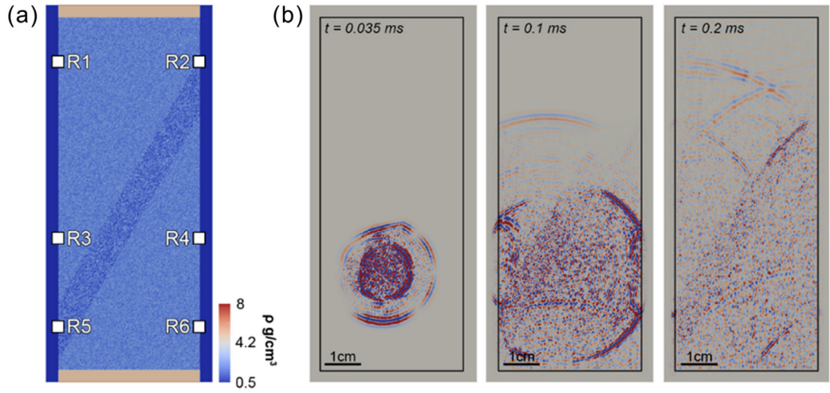
Figure 3.6: Simulation of the wavefield trapped within the fault network structure and increasing drastically peak delays at near-fault receivers, redrawn from King et al. (2023).
