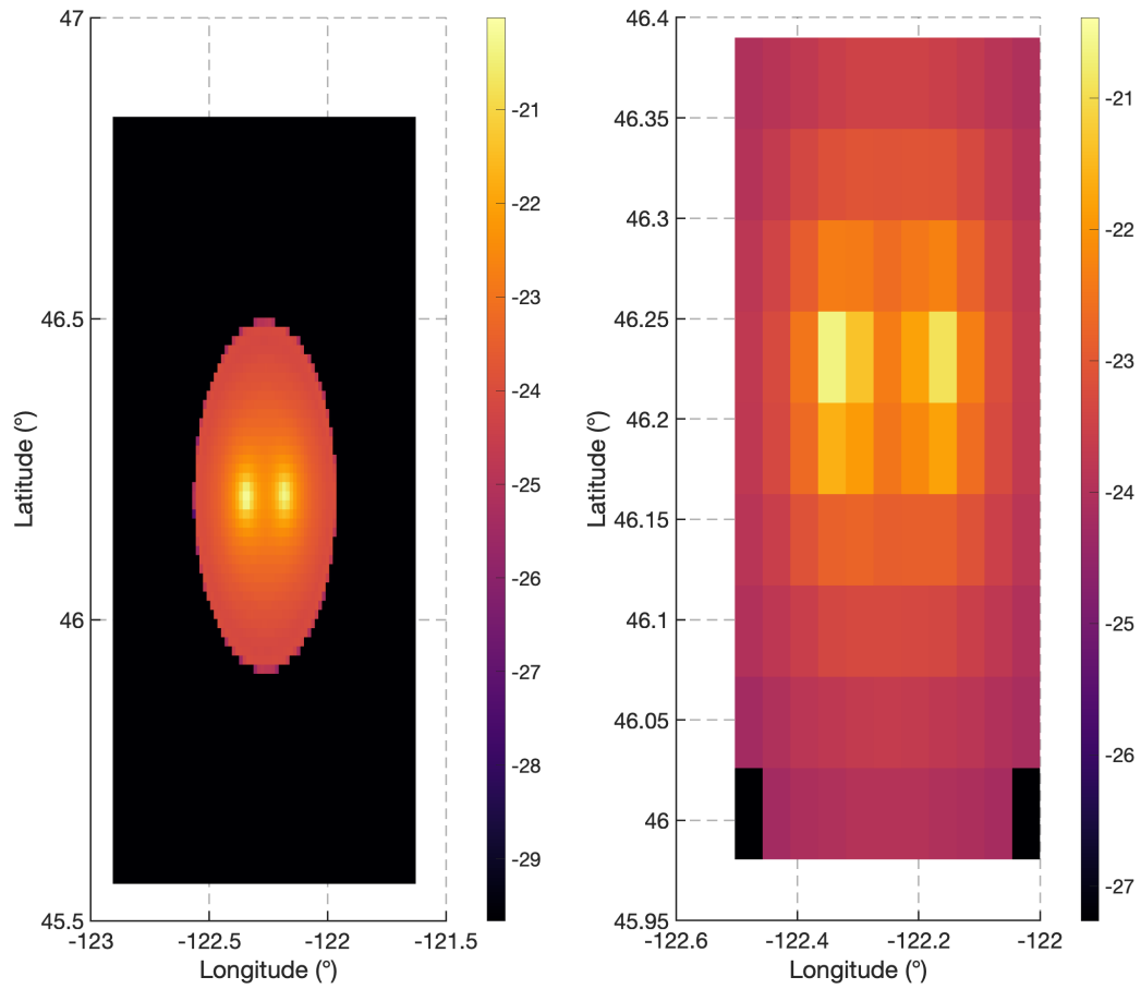
Figure 10.3: Kernels for coda-attenuation imaging at 3 Hz for the MSH dataset. The full kernels are shown as a section in the 3D space (a) and in the grid chosen for the inversion (b). Notice that sensitivity is always highest at the source and receiver. The colour scale is logarithmic. The lapse time is 22.5 s.
