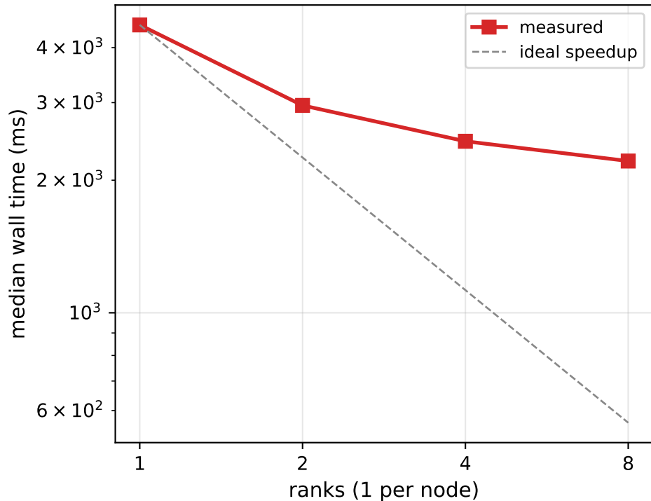
MPI strong scaling — medium ( 256^3 )
