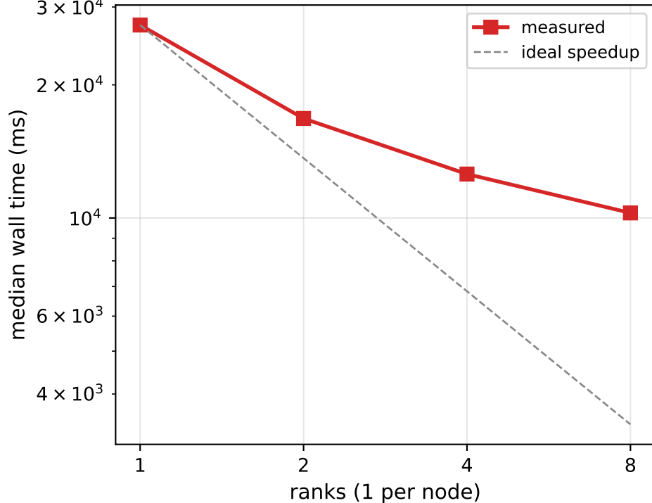
MPI strong scaling — large ( 512 \times 512 \times 256 )
