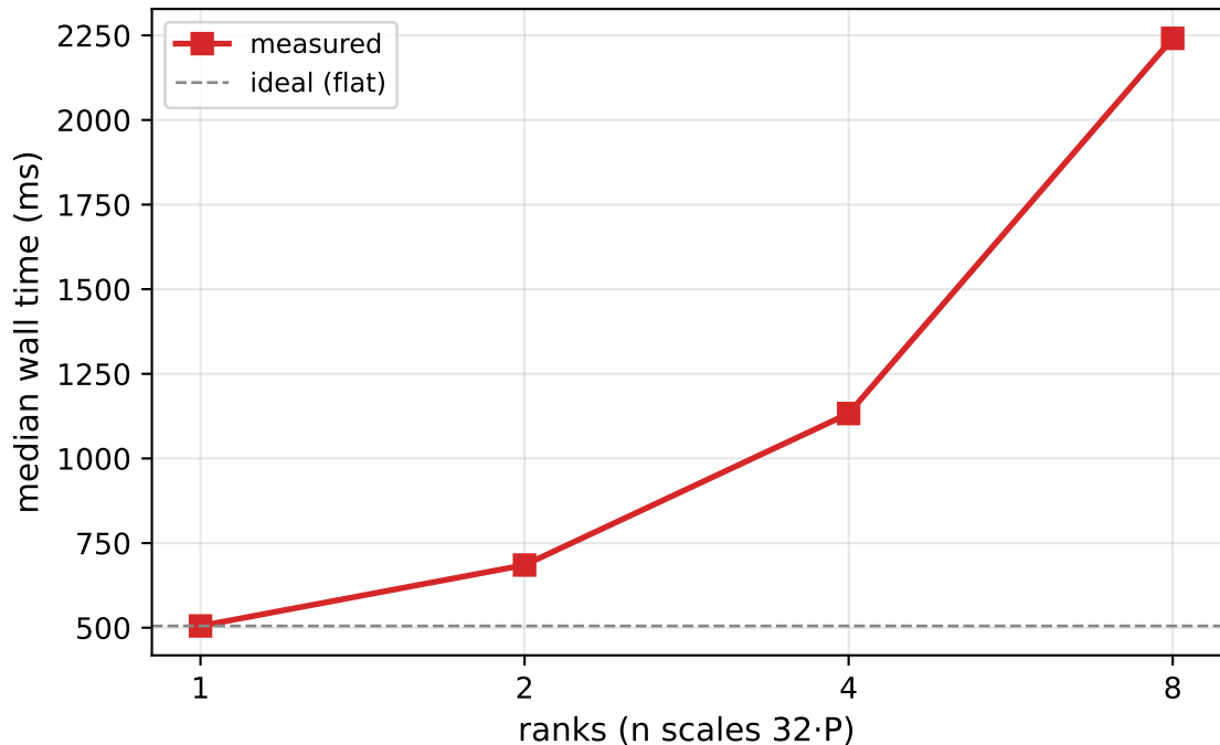
MPI weak scaling (256×256×n)
