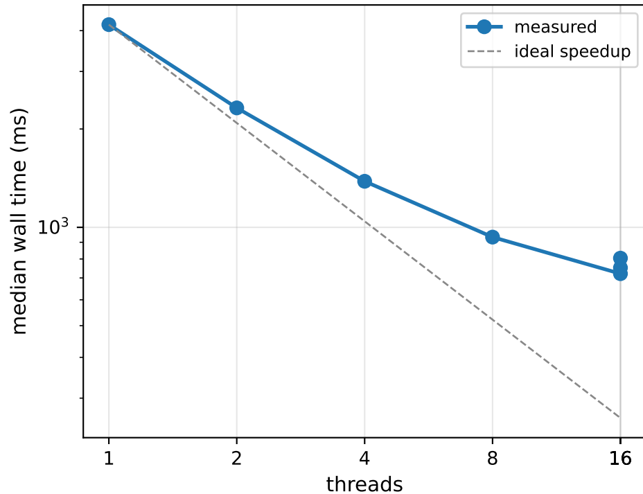
OpenMP strong scaling — medium ( 256^3 )
