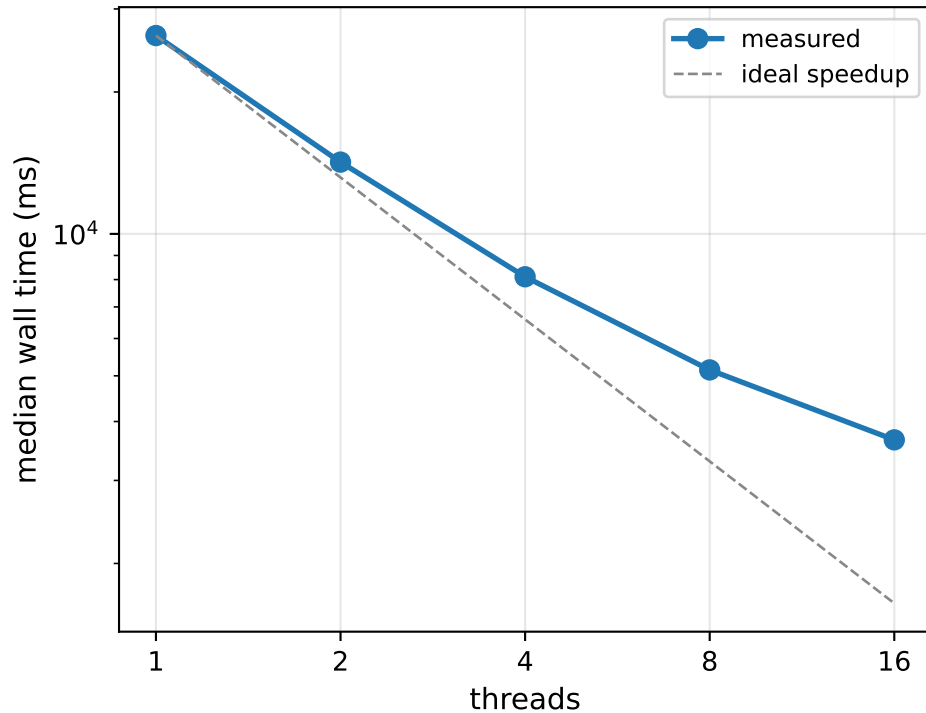
OpenMP strong scaling — large ( 512 \times 512 \times 256 )
