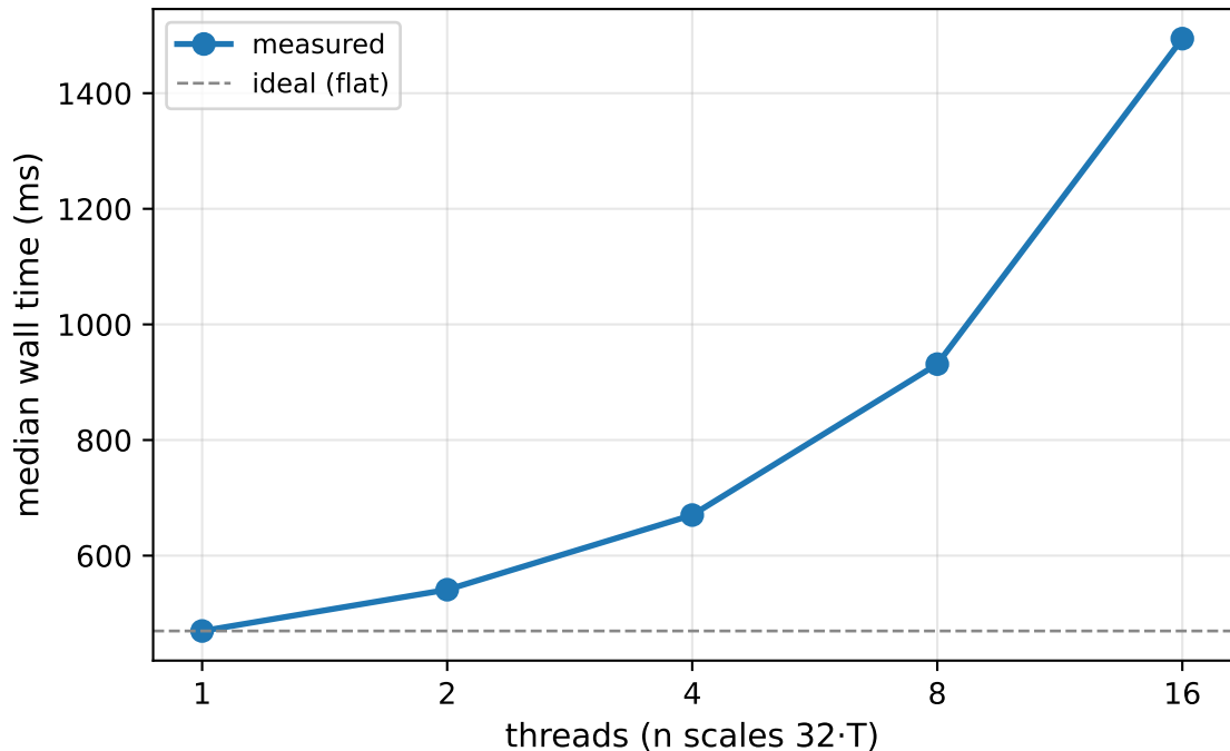
OpenMP weak scaling (256×256×n)
