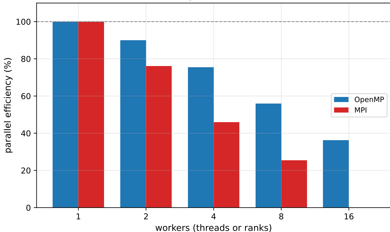
Parallel efficiency at medium fixture ( 256^3 )
