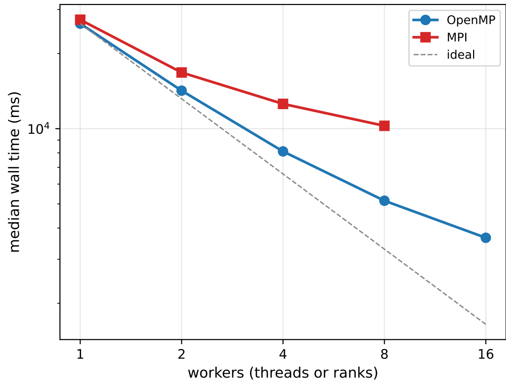
Strong scaling — large ( 512 \times 512 \times 256 )
