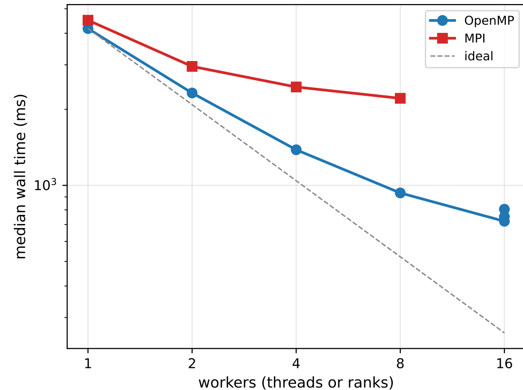
Strong scaling — medium ( 256^3 )
