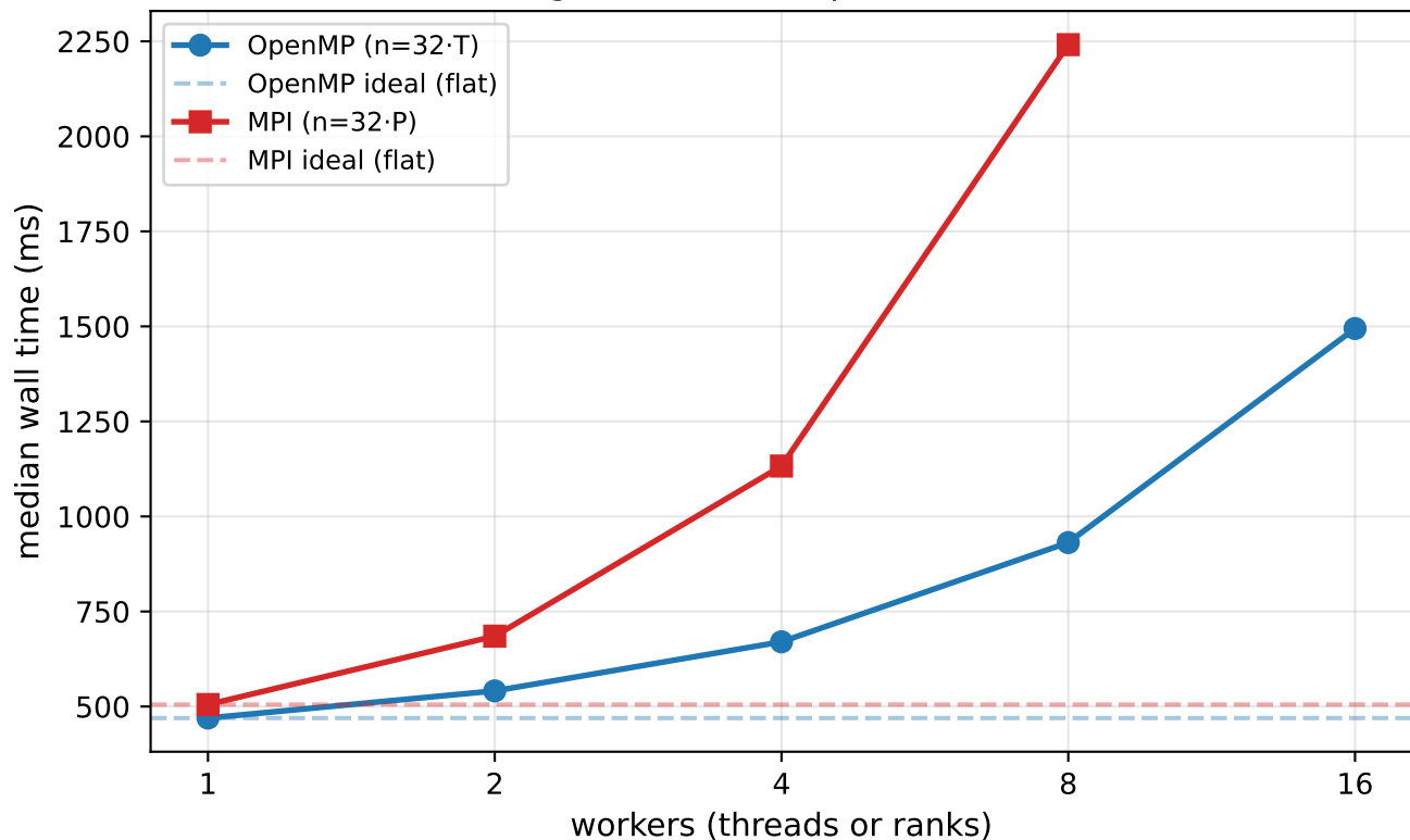
Weak scaling (256×256×n, per-worker work fixed)
