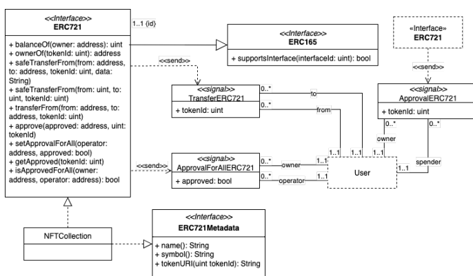
Fig. 4. UML Class Diagram of a NFT.
