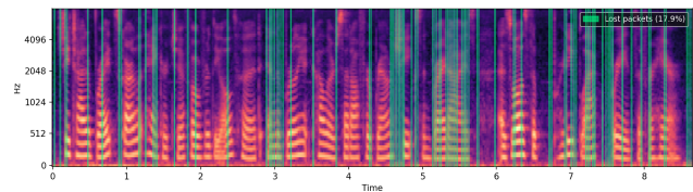
Figure 1. Spectrogram of a speech signal corrupted by simulated packet loss (Gilbert-Elliott model, overall loss rate 17.9%). Green vertical lines mark lost packets, each corresponding to a 15ms audio frame. Note the bursty nature of the losses: packets tend to drop in clusters rather than in isolation, reflecting the two-state Markov structure...
