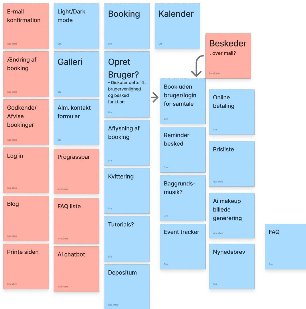
Figur 31: Features.
