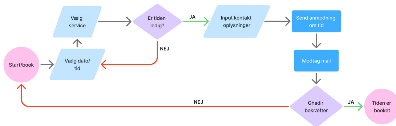
Figur 35: Flowchart.
