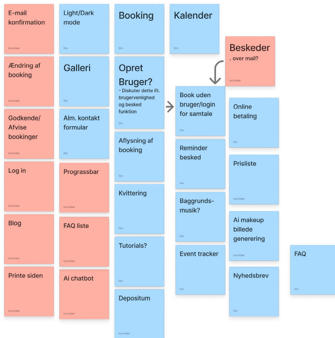
Figur 31: Features.
