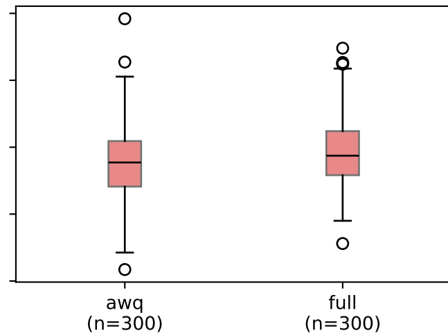
quantization
