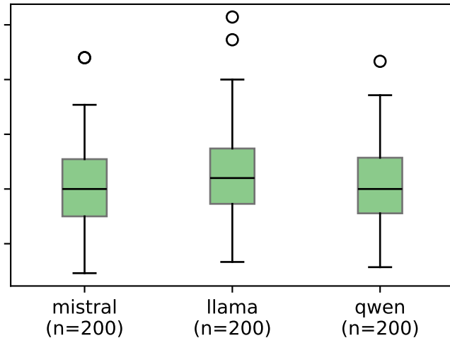
model
