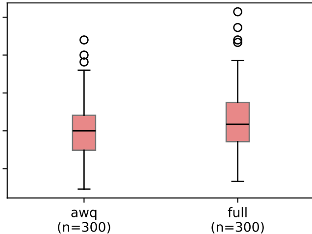
quantization
