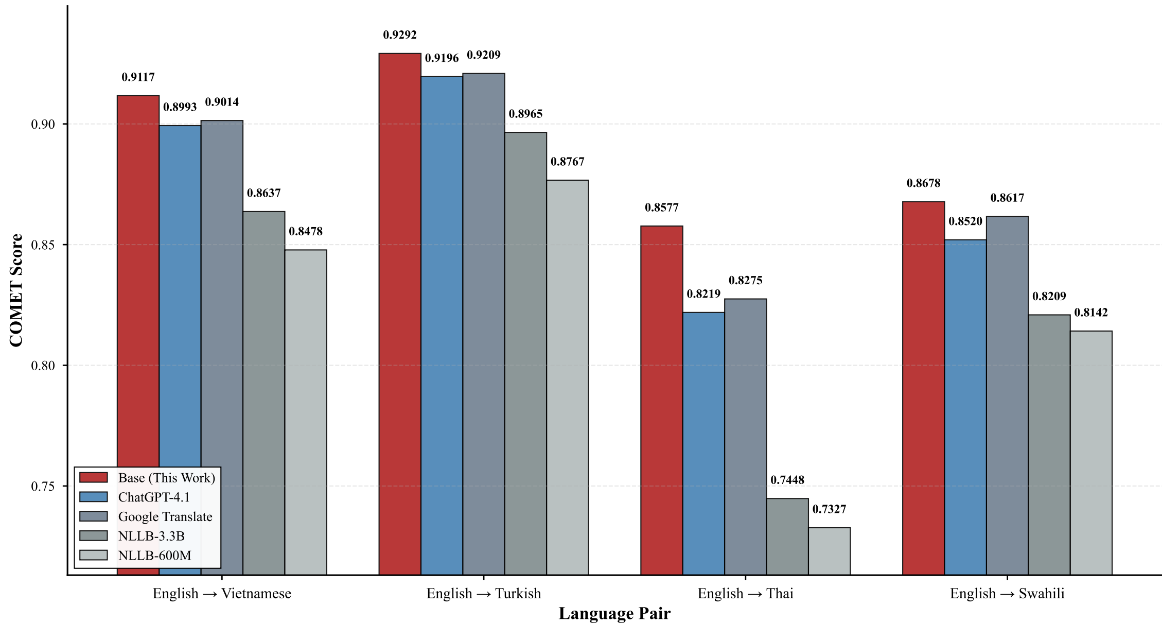
COMET Score Comparison Across Translation Systems
