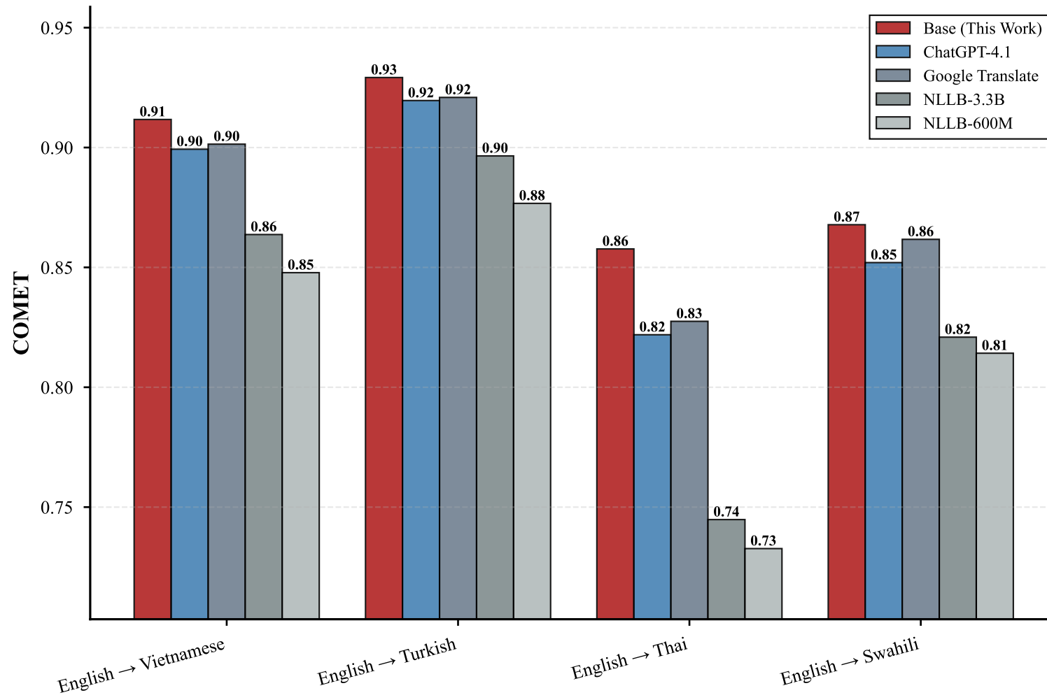
COMET Score
