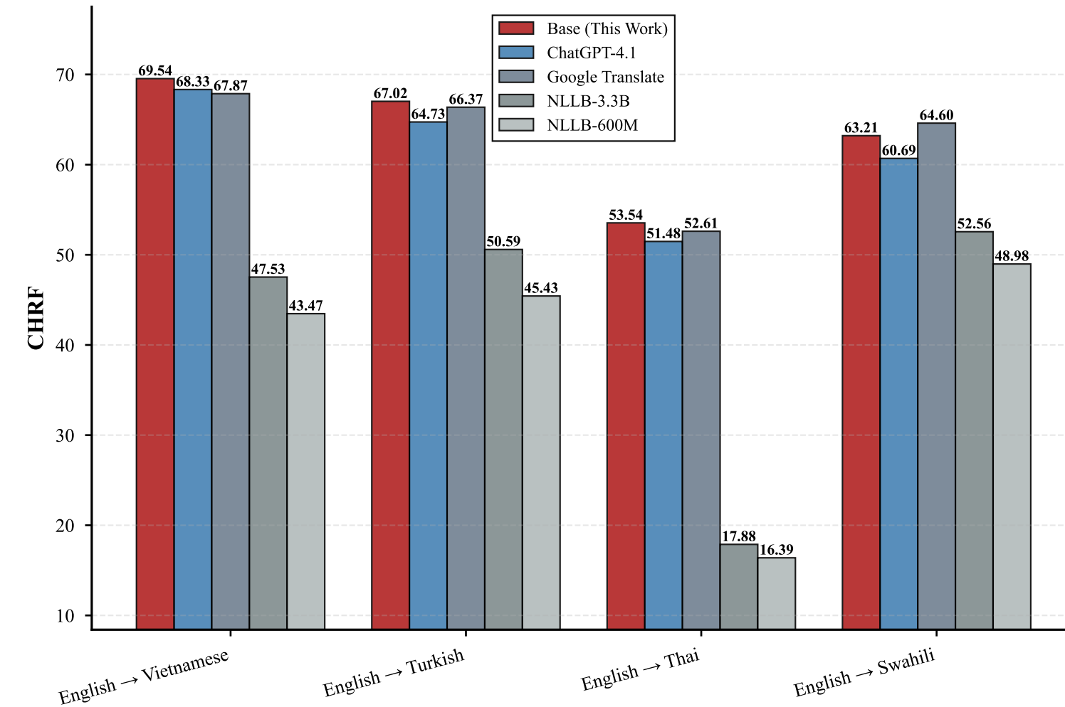
chrF Score
