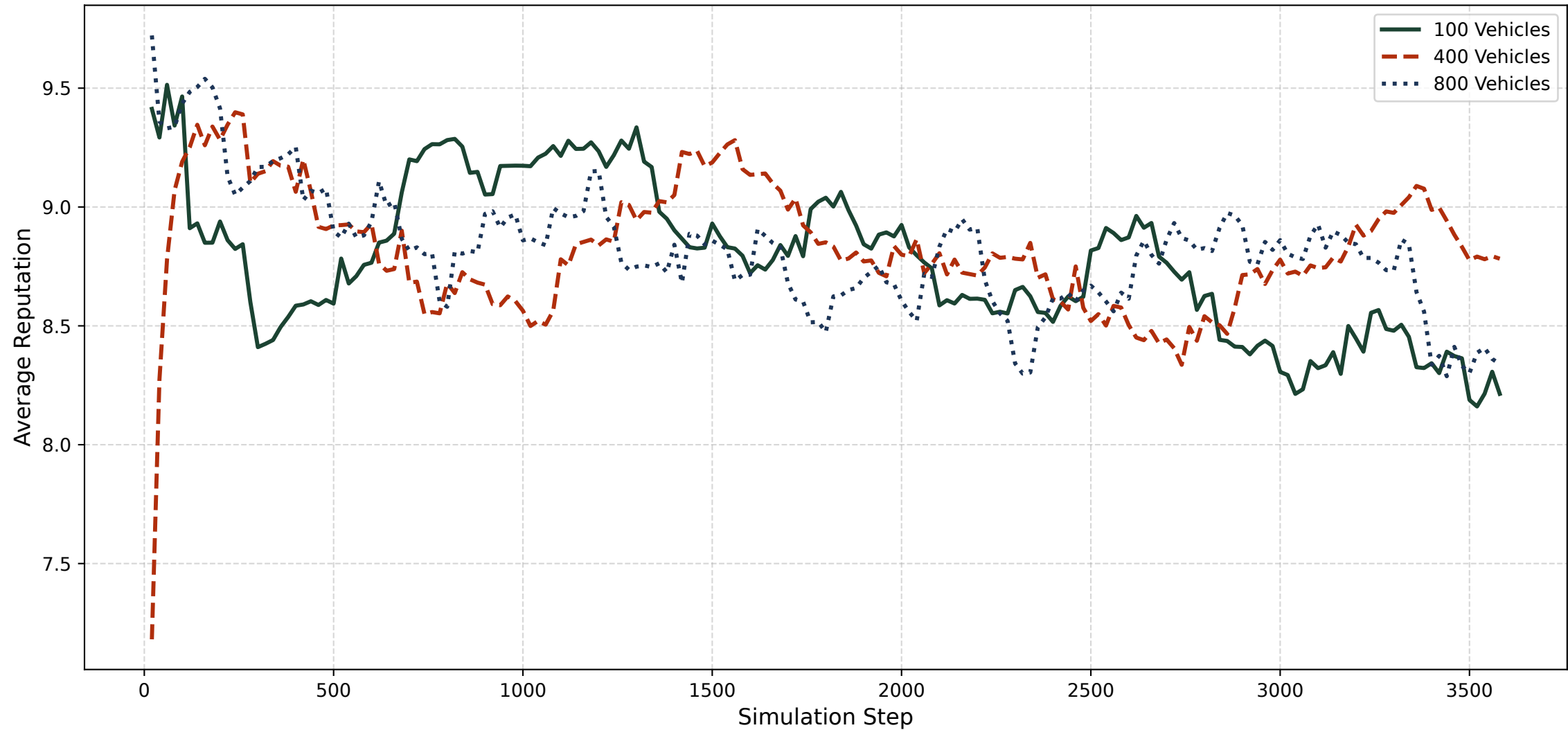
Reputation Evolution Across Traffic Densities
