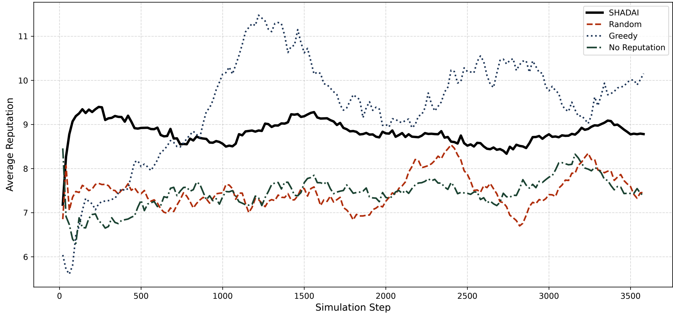
Average Reputation Comparison Across Selection Strategies
