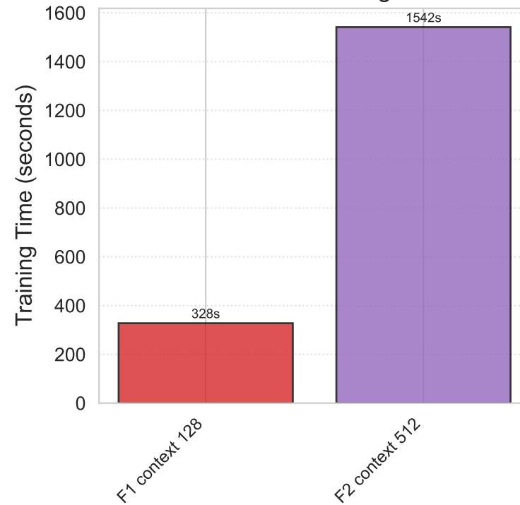
F: Context Length
