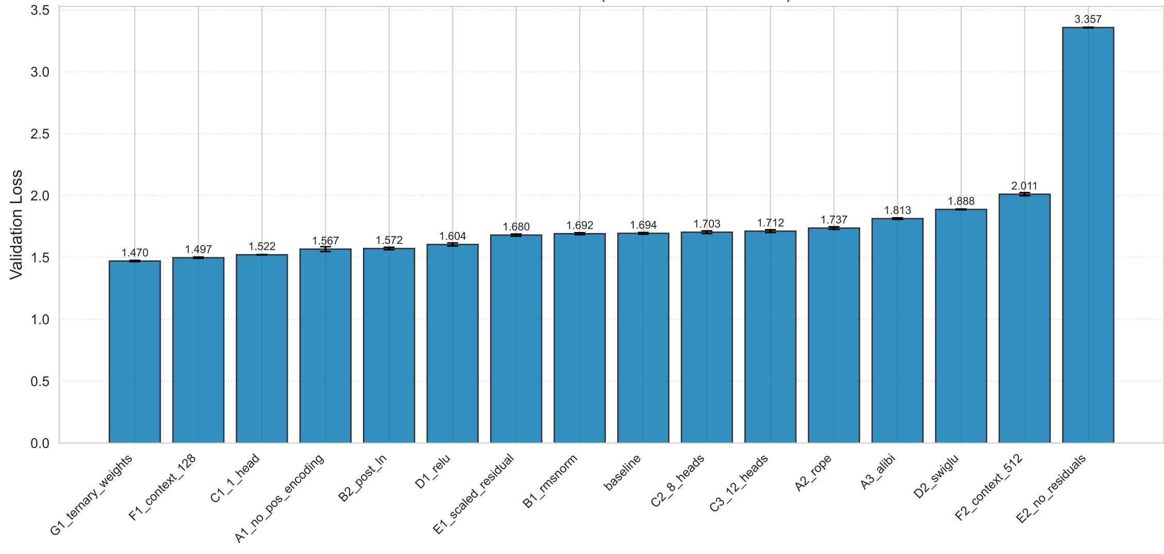
Final Validation Loss (mean \pm std over seeds)
