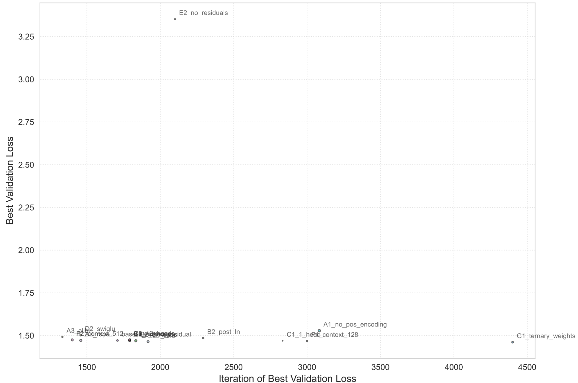
Convergence Speed vs. Best Performance (bubble size = std)
