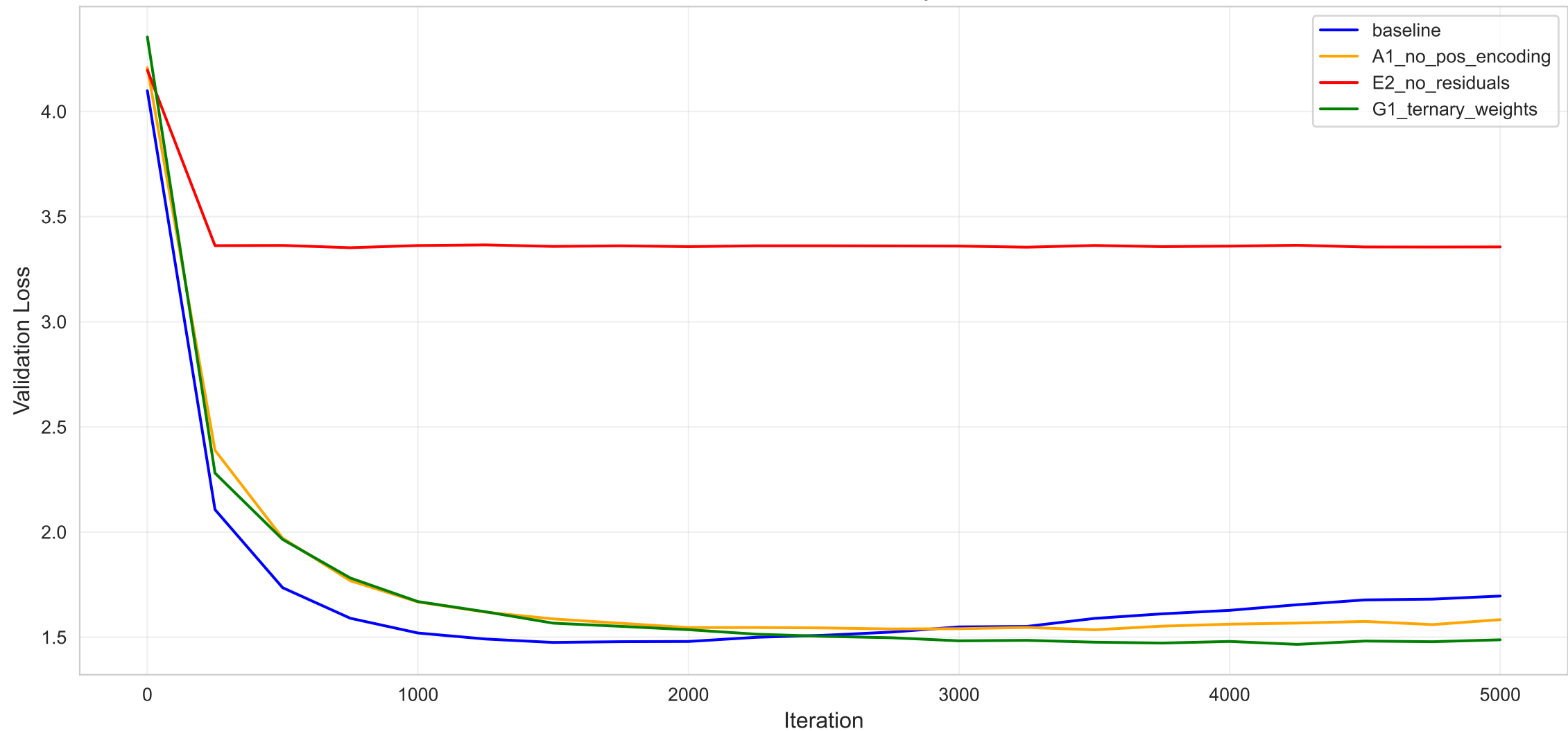
Validation Loss Curves for Key Ablations
