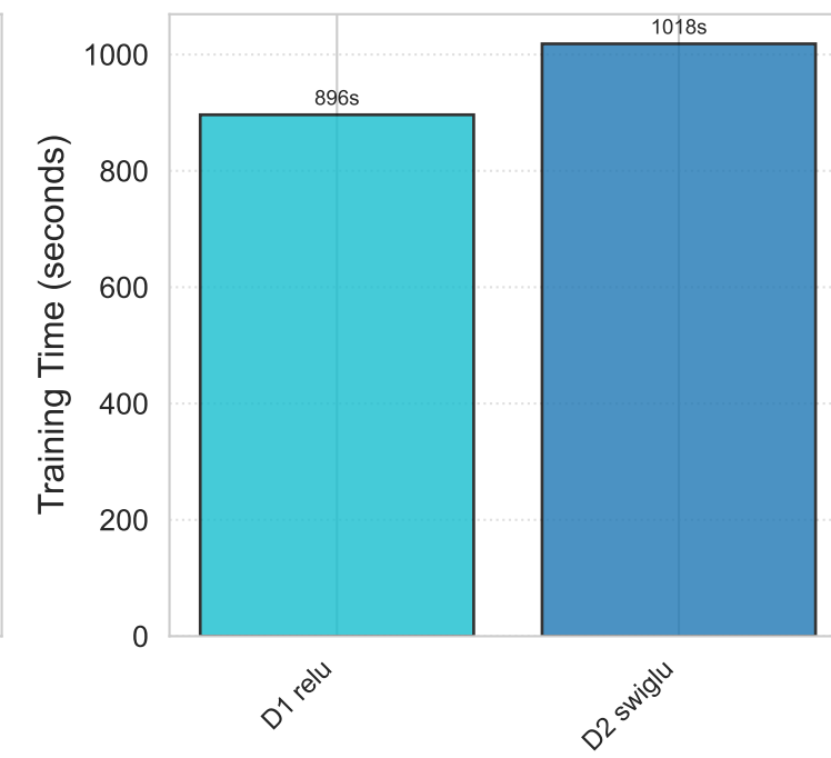
D: Activation
