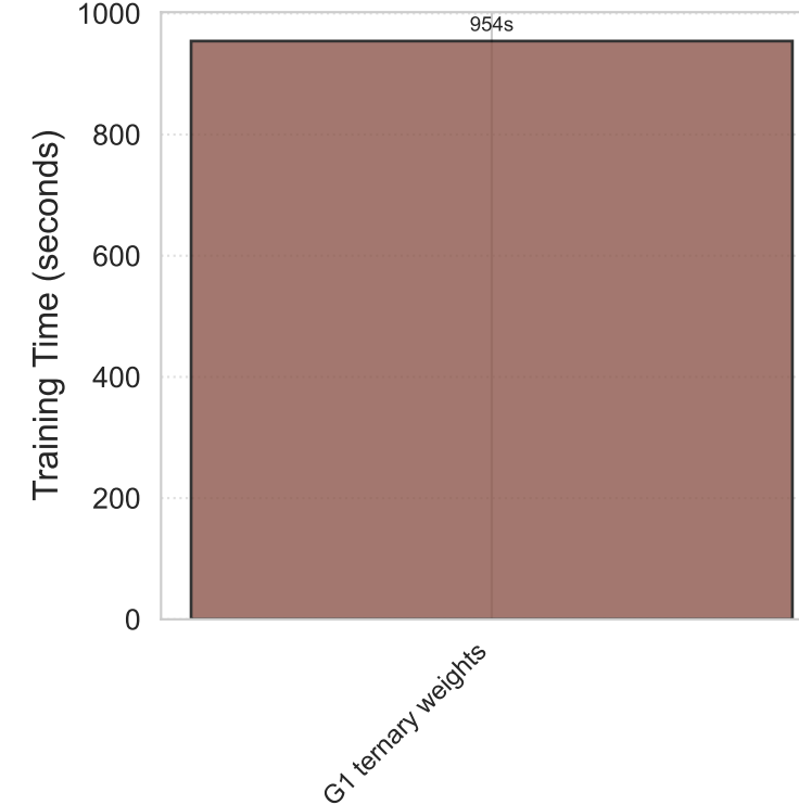
G: Quantization
