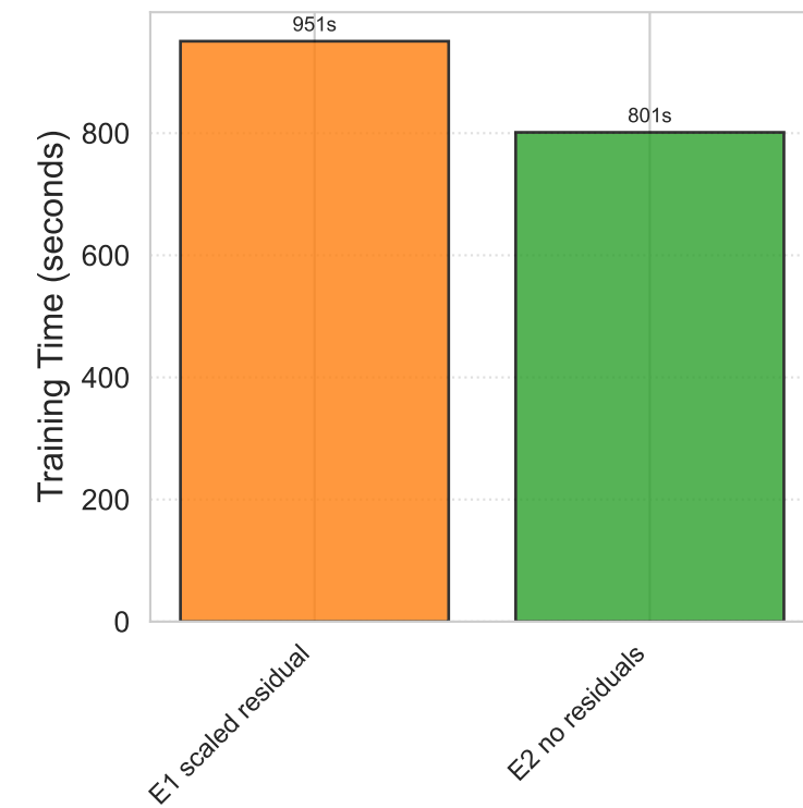
E: Residual
