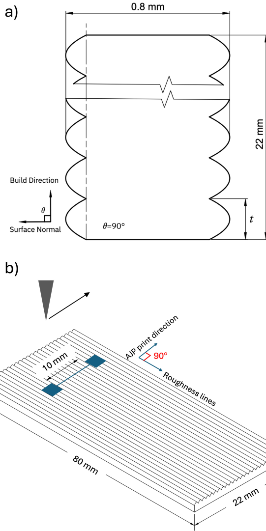
Fig. 2 Overview of the experimental setup showing (a) the FDM surface roughness profile and (b) the pattern design and print orientation relative to the substrate topography.
