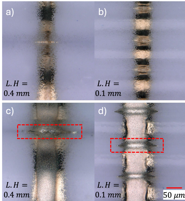
Fig. 5 Optical microscopy images of AJP-printed lines on rough substrates under two deposition conditions: (a–b) baseline parameters (Test Condition 3, carrier gas flow rate 8 sccm and sheath gas flow rate 50 sccm) and (c–d) higher deposition rate (carrier gas flow rate 20 sccm and sheath gas flow rate 40 sccm) with constant print speed and stand-off distance, for L.H. = 0.1 mm and 0.4 mm. Higher deposition rate preserves continuity at L.H. = 0.4 mm but increases line width and material accumulation within surface grooves (red rectangles). All images are shown at identical magnification.
