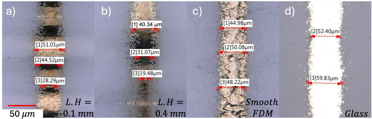
Fig. 6 Line width measurements for representative substrates with varying surface roughness.
