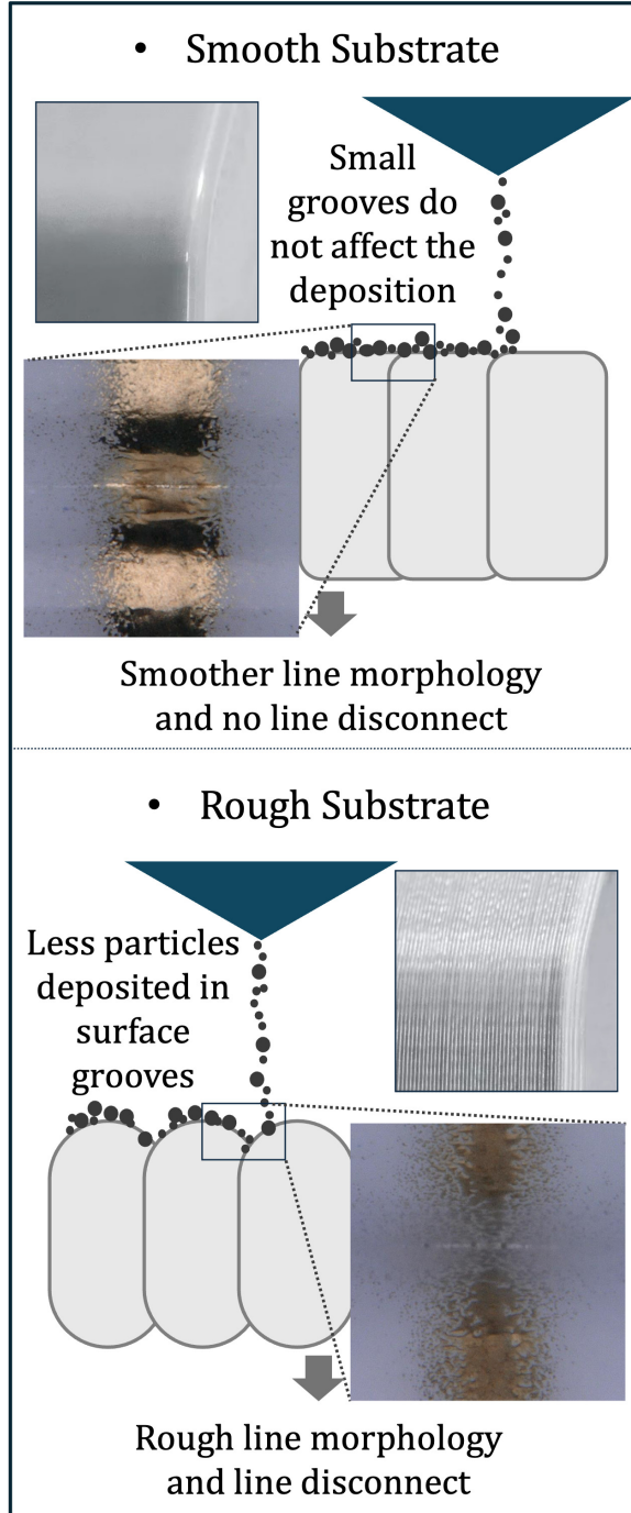
Fig. 1 Schematic illustration of the effect of surface roughness on AJP particle deposition. On a smooth surface, the particles form a continuous trace. On a rough surface, deposition in the valleys is incomplete, resulting in partial disconnections and reduced trace continuity.
