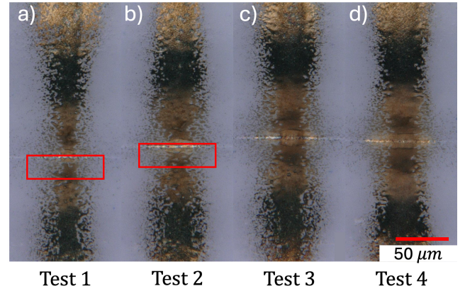
Fig. 4 High-resolution microscopy images of AJP lines printed on an FDM substrate with 0.3 mm layer height under four process conditions.
