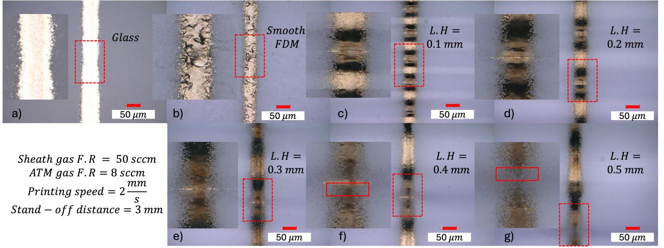
Fig. 3 Microscopy images of AJP-printed silver traces on glass, smooth FDM, and FDM substrates with varying layer heights.
