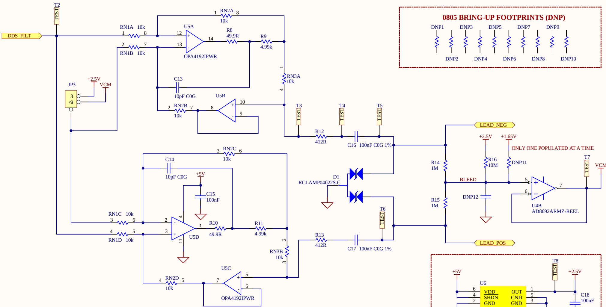
MIRRORED ENHANCED HOWLAND CURRENT PUMP
