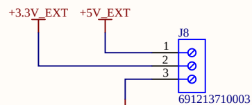
EXTERNAL POWER
