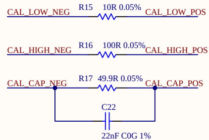
CALIBRATION LOADS
