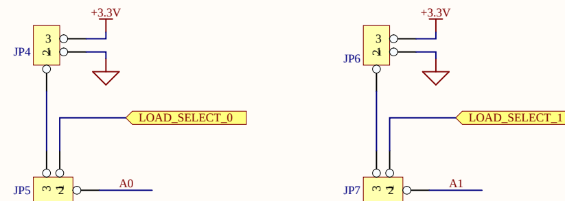
LOAD SELECTOR SOURCE SWITCH
