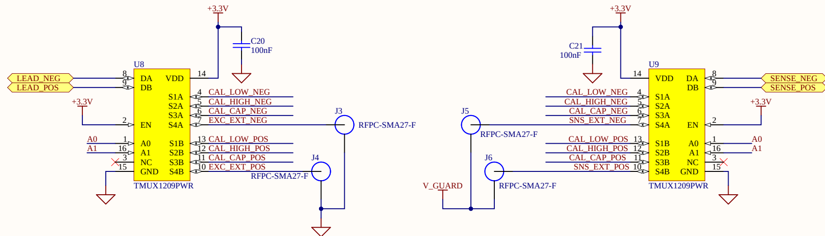
LOAD SWITCHES & EXTERNAL CONNECTORS
