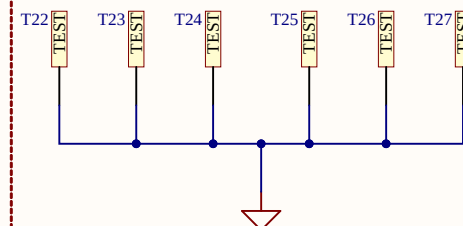
REFERENCE TEST POINTS
