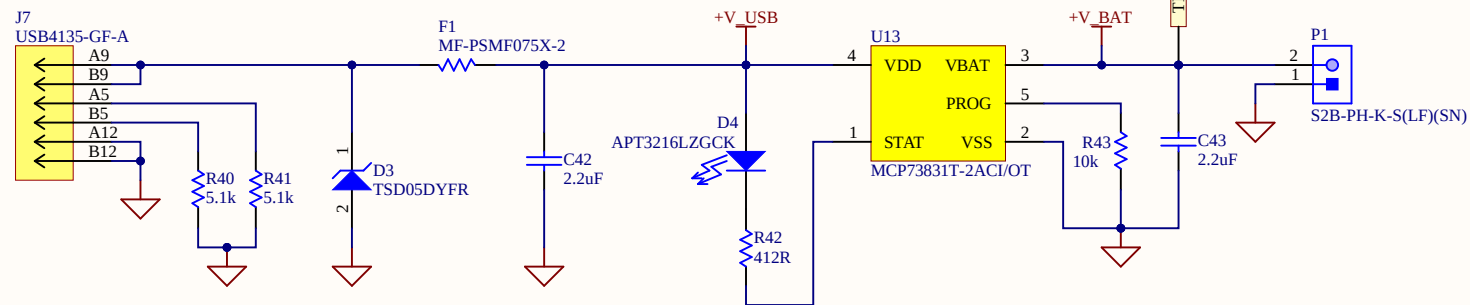
LIPO BATTERY MANAGEMENT WITH USB-C CONNECTOR
