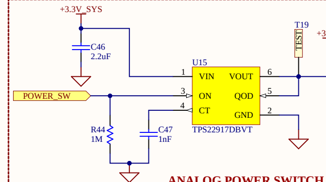
ANALOG POWER SWITCH
