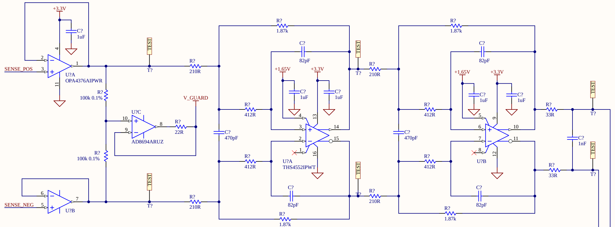
BUFFER STAGE
