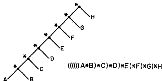
a) TREE YIELDING MINIMUM NUMBER OF REGISTERS
