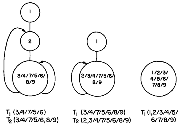
Figure 6. Collapsibility—Repeated Applications of Two Transformations Yield a Single Node in O(n \log n) Steps
