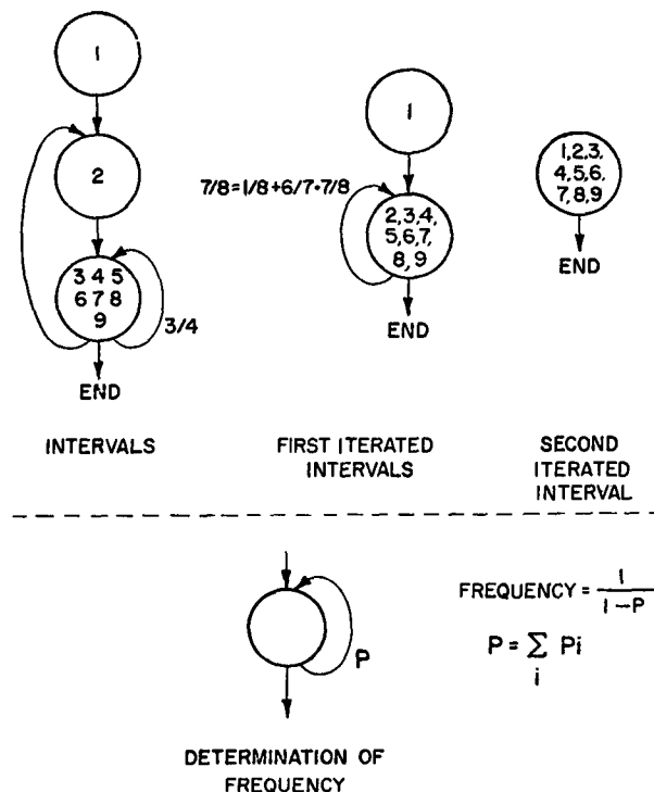
Figure 5. Interval Analysis and Frequency Determination—Relative Frequency of a Loop May Be Determined from the Probability of a Loop-Closing Branch
