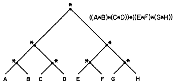
a) TREE YIELDING MINIMUM NUMBER OF REGISTERS
