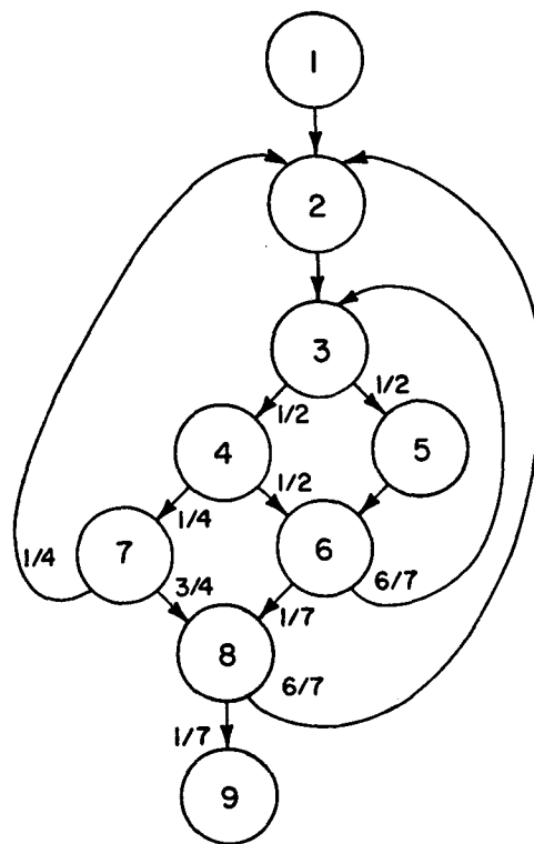
Figure 4. Program Flow Graph with Branch Probabilities
