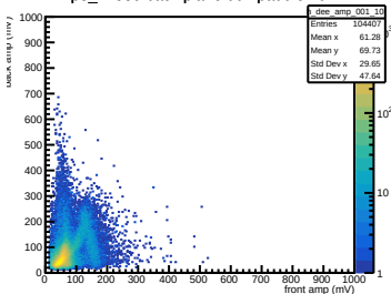
p3_22536 back plane 001 paddle 10
