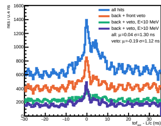
H plane 101 bar 0
