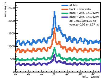
P plane 101 bar 8
