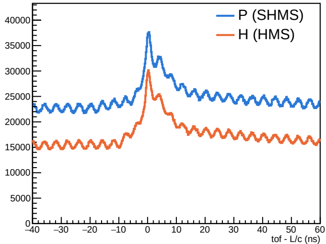
all hits: P (SHMS) vs H (HMS)
