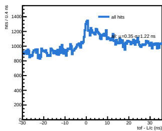
P plane 200 bar 9
