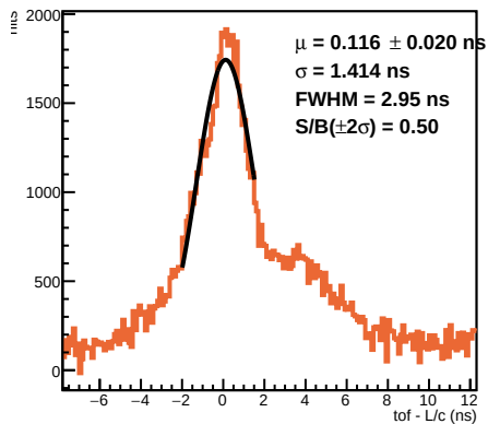
P back + front veto [tofcrf], bg-subtracted
