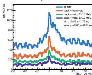
H plane 101 bar 6
