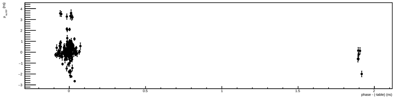
H: photon peak without RF vs RF phase - table (run groups)
