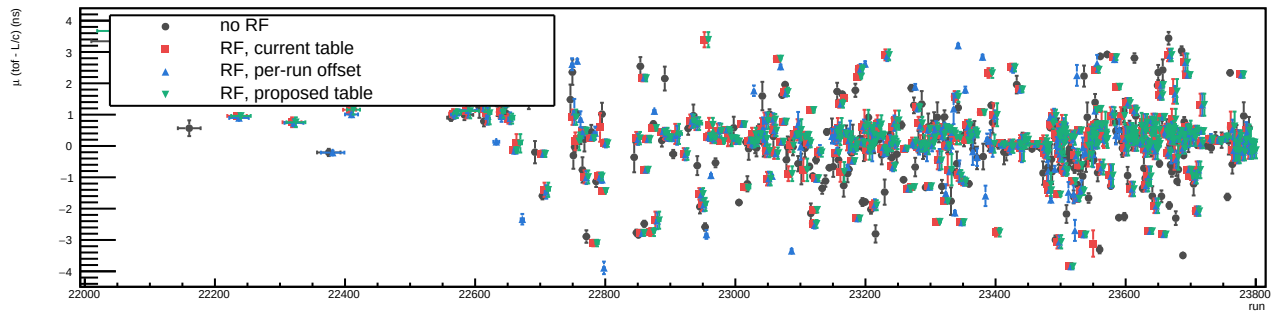
P: photon peak per run group (width fixed)
