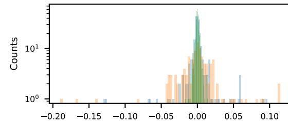
fDCAxyTrk1KF
