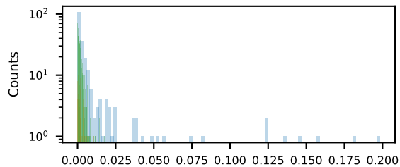
fDCAxyBetweenTrksKF
